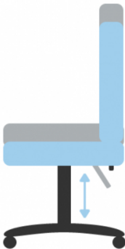
Gas Lift Height Lever
